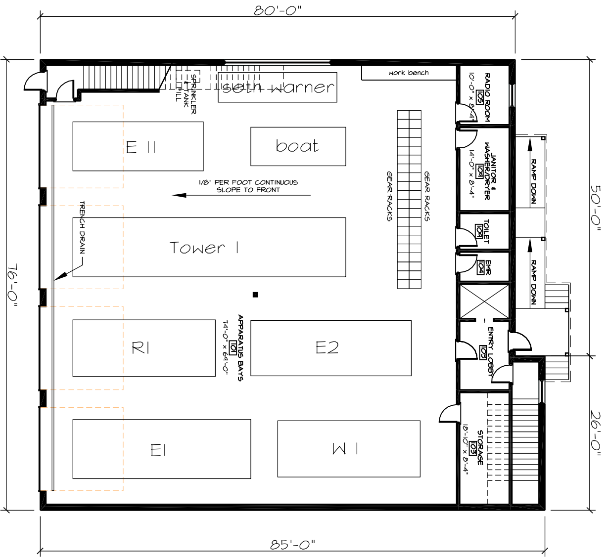
FIRST FLOOR PLAN 1/16" = 1'-0" 6,210 SF
