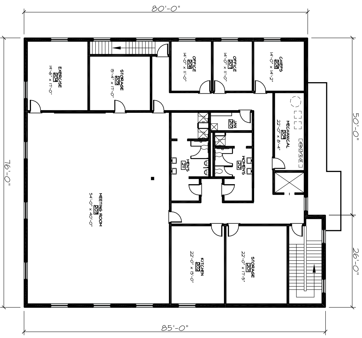
SECOND FLOOR PLAN 1/16" = 1'-0" 6,210 SF
